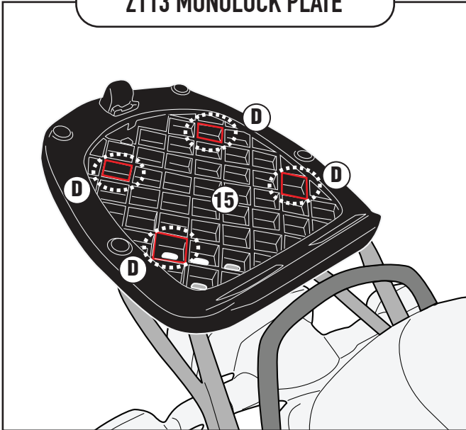
Z113 MONOLOCK PLATE
