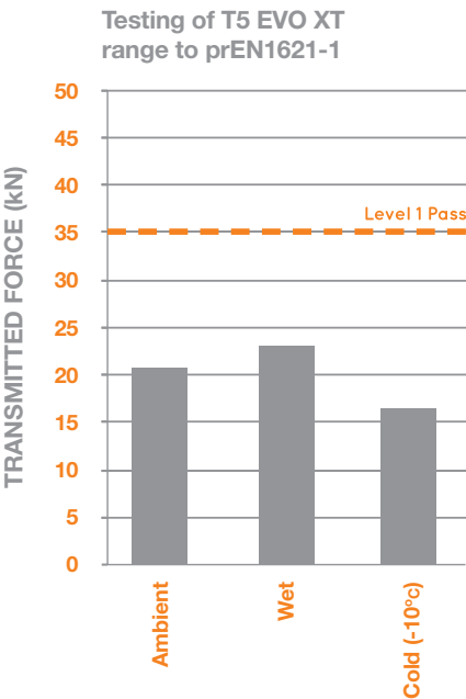
SAMPLE CONDITIONING
